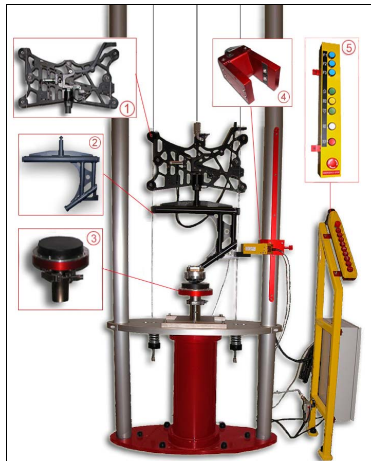
Twin Wire Machine -Bottom
