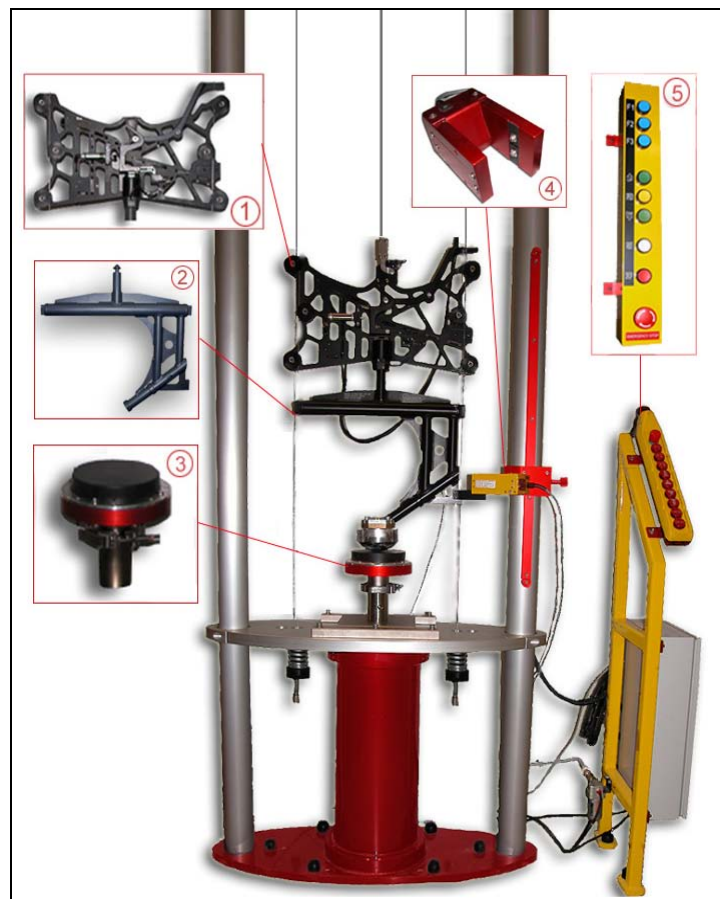
Twin Wire Machine -Bottom
