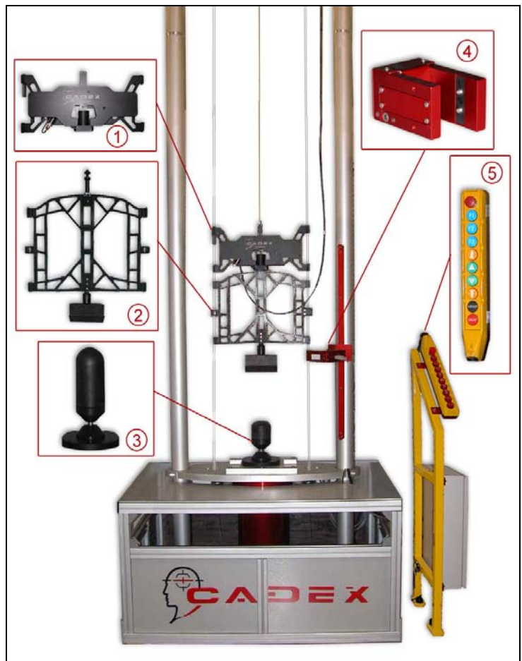
Twin Wire 1000 Kg Machine - Bottom
