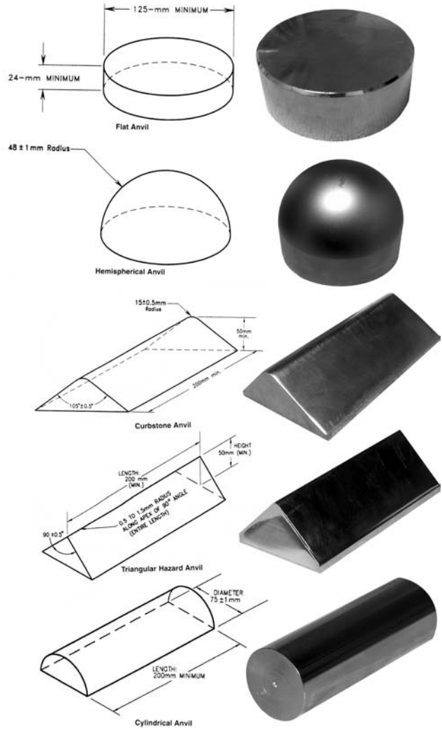
Anvils for all existing standards are available.
