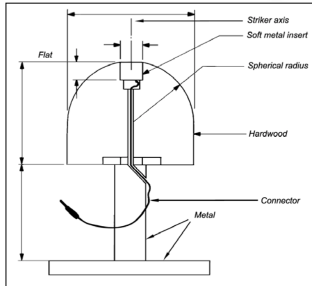
Test block for testing penetration resistance.
