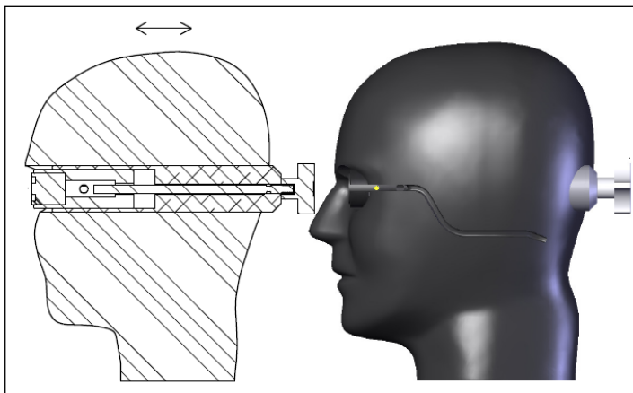
Depth adjustment device for sensor
