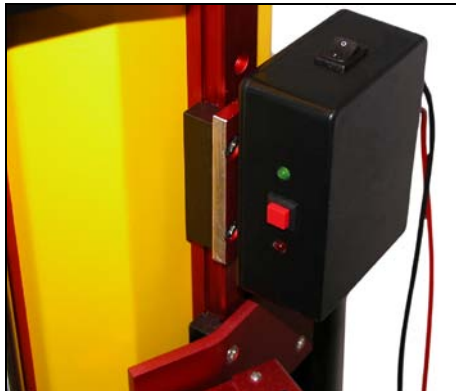
Front view, installed on a monorail.
