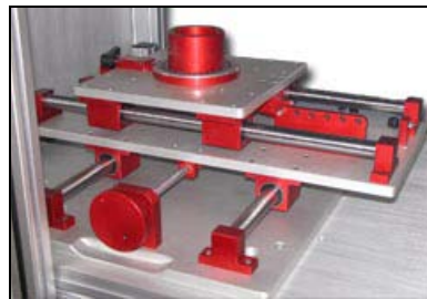
Motorized holding table
